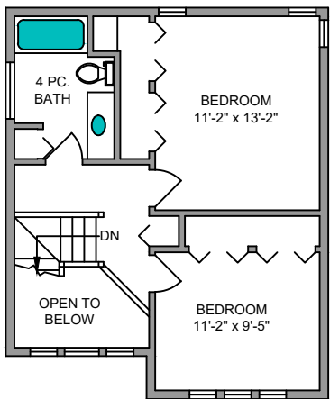
UPPER FLOOR 500 SQ. FT. 8' CEILING HEIGHT
